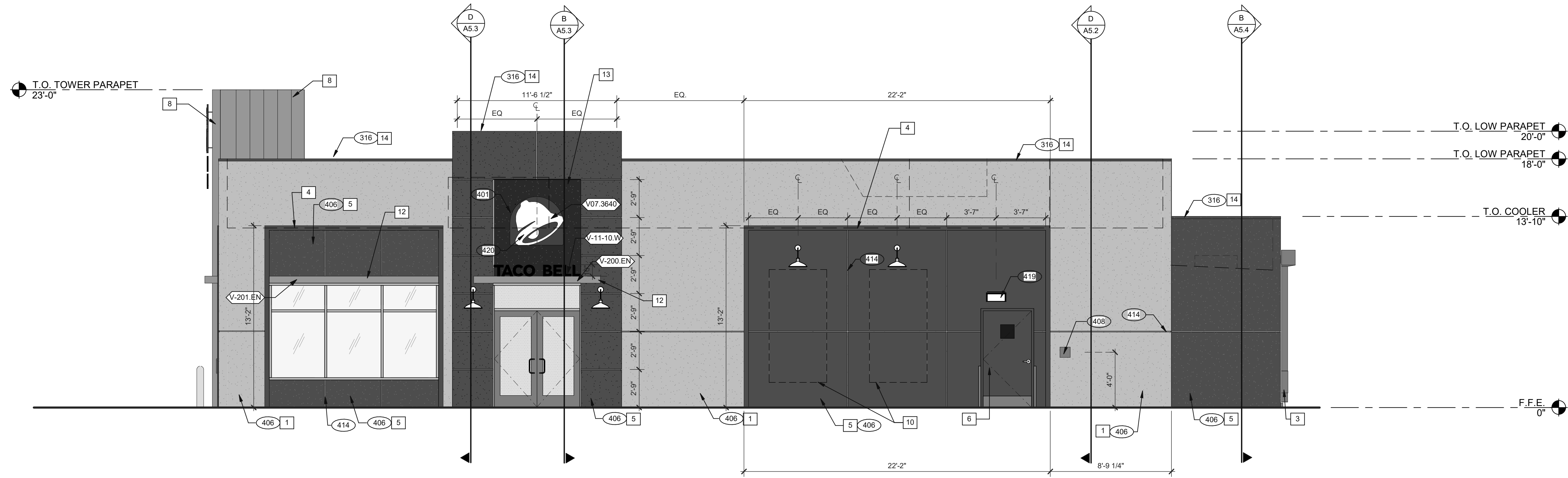
FRONT ELEVATION 1/4" = 1'-0" 1
