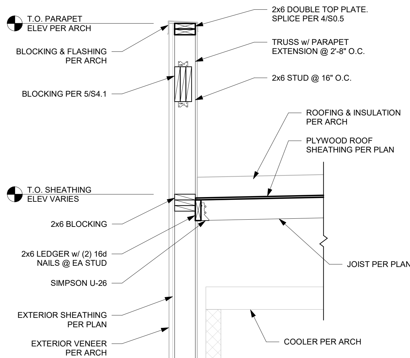
3 SECTION S4.3 3/4" = 1'-0"
