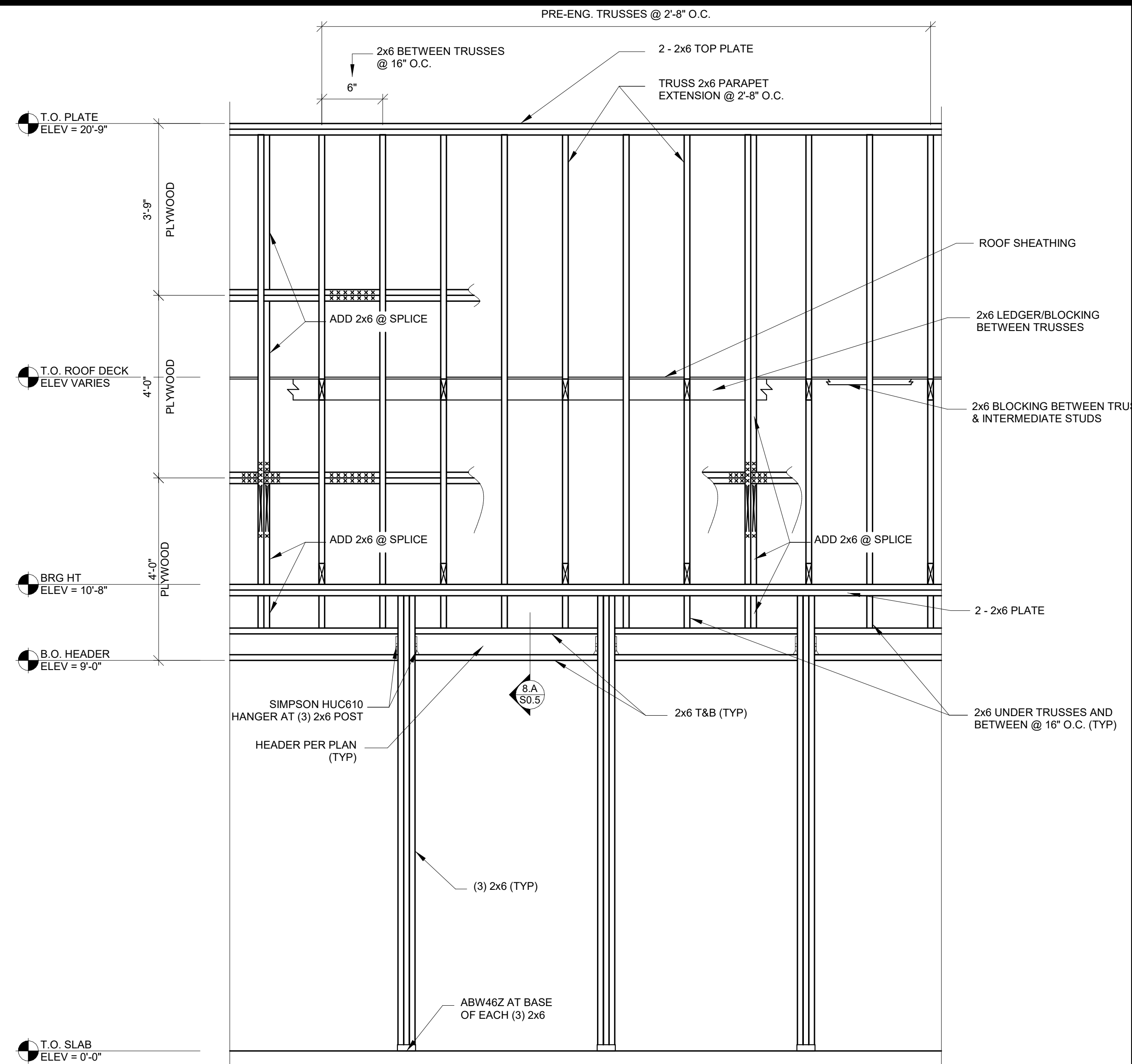
4 SECTION S4.3 1 1/2" = 1'-0"
